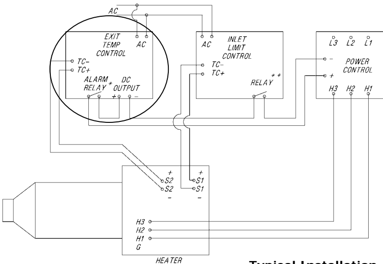
Typical Installation with SureHeat MAX
